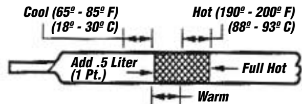
Figure 2 Filling Transmission
